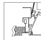
Tegular detail
