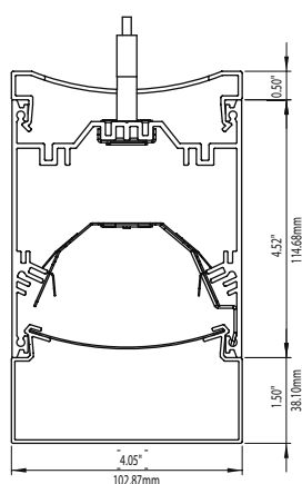
1.5" Pop-Down Lens
