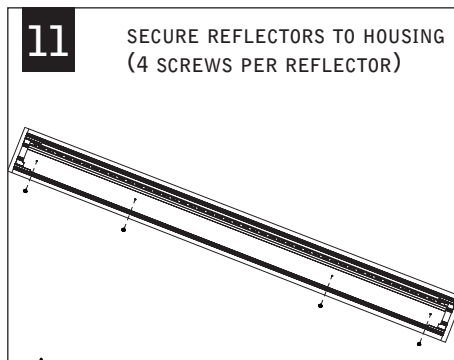
SECURE REFLECTORS TO HOUSING (4 SCREWS PER REFLECTOR) ⚠ AVOID ALL CONTACT WITH LED SURFACE, LEDs ARE EASILY DAMAGED!
