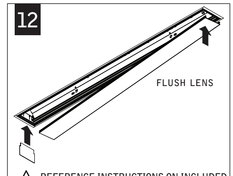
FLUSH LENS ⚠ REFERENCE INSTRUCTIONS ON INCLUDED TOOL FOR LENS INSTALLATION.
