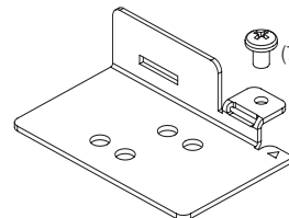
Joiner Bracket Assembly (A11623-01)
