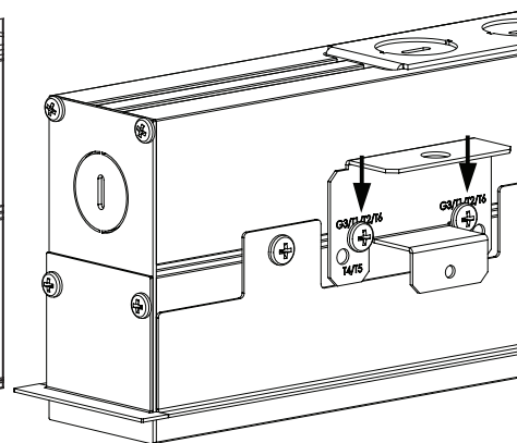
G3: 9/16" Slot-Tee Tegular Tile T1: STD 15/16" Tegular Tile T2: STD 9/16" Tegular Tile T4: Tall 15/16" Tegular Tile T5: Tall 9/16" Tegular Tile T6: 9/16" Node Tegular Tile
