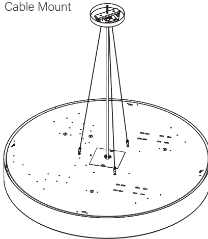
Cable Mount
