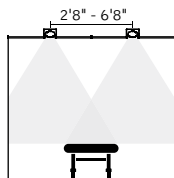
Ambient distribution
