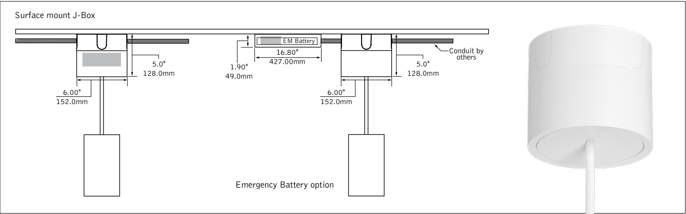
DPC - Power Canopy with decorative J-box cover
