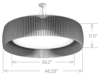
48" Shade | 3' Light Engine | 12" Height
