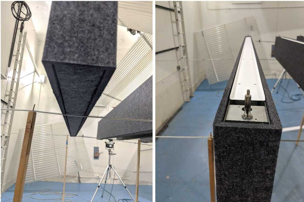
Figure 2 – Individual object, faces oriented toward (left) and away from (right) horizontal test surface
