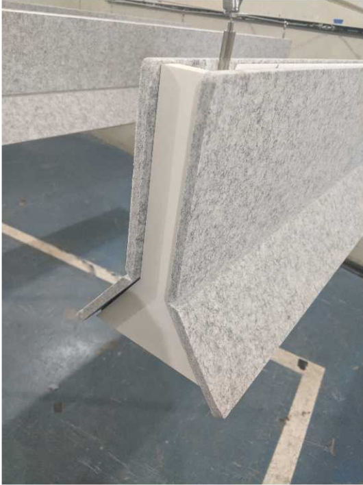
Figure 3 – Detail of specimen geometry and materials
