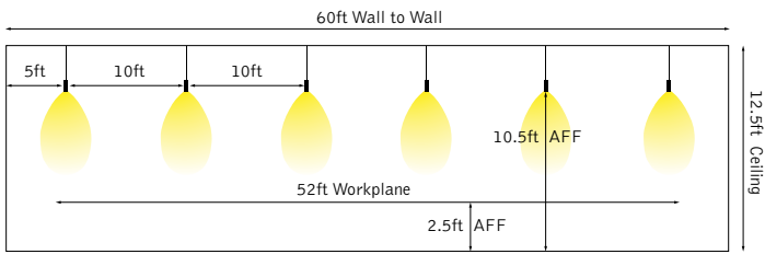
Workplane Illuminance
