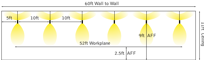
Workplane Illuminance
