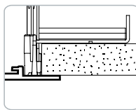
ceiling cutout dimensions: T & IC Housings - 4 11/16" RT Housing - 4 5/8"
